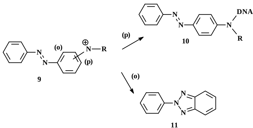
Fig. 16. Reaction pathways for type 9 nitrenium ion metabolites of azobenzene isomers
