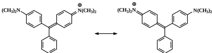
Fig. 4. A pair of resonance structures for Malachite Green (C.I. Basic Green 4)
