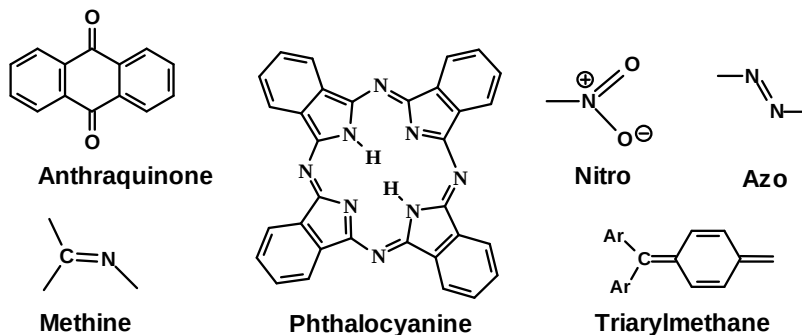
Fig. 2. Examples of chromophoric groups present in organic dyes
