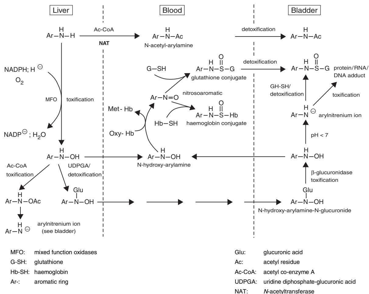
Fig. 1: Metabolism of primary aminoaromatics: formation and transport of the detoxification stages in the various compartments (40)
