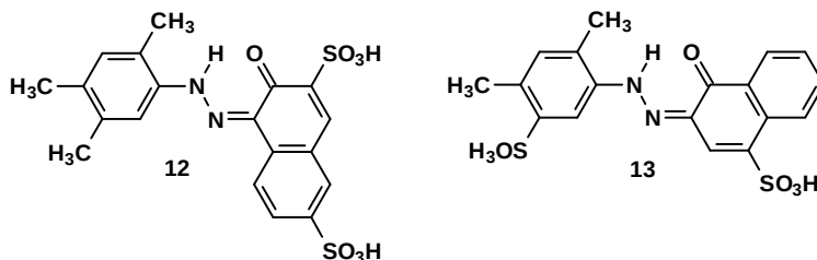
Fig. 17. Carcinogenic (12) and noncarcinogenic (13) water-soluble monoazo dyes
