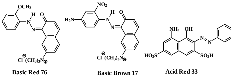
Fig. 20. Examples of non-permanent hair dyes
