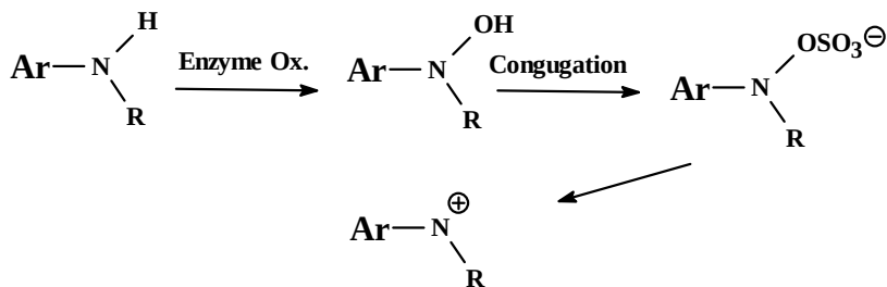
Fig. 15. Nitrenium ion formation from the metabolism of aromatic amines
