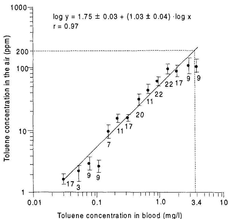
Fig. 2: Relationship between external and internal toluene exposure under workplace conditions ( n = 183 )
