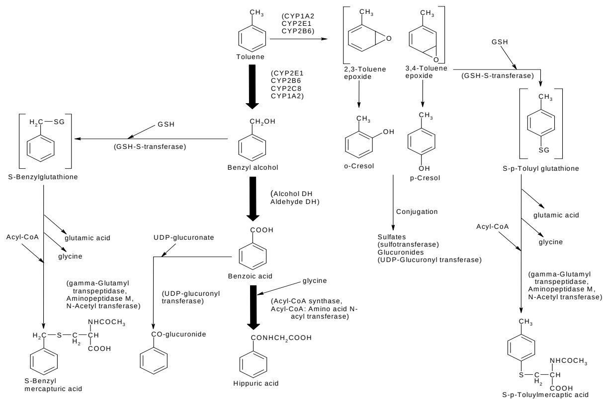
Figure 1. Proposed pathways for toluene metabolism.*, **
