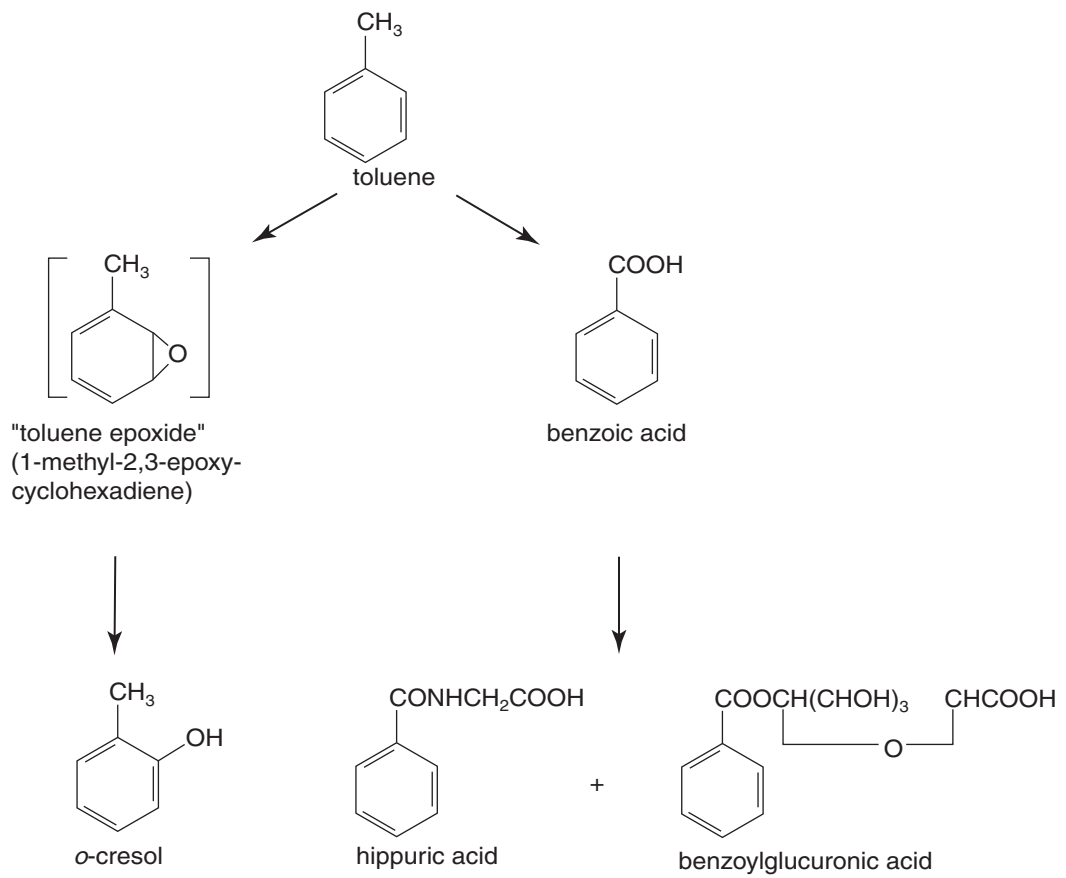
Fig. 1: Metabolism of toluene in humans
