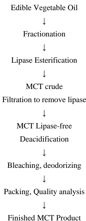
Figure 3. Caprylic/Capric Triglyceride (MCT) production scheme
