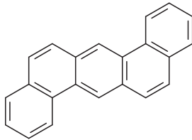
dibenz[a,h]anthracene
